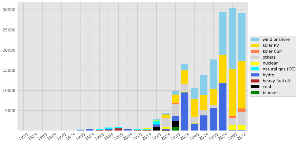
Power plant new capacity (MW)
