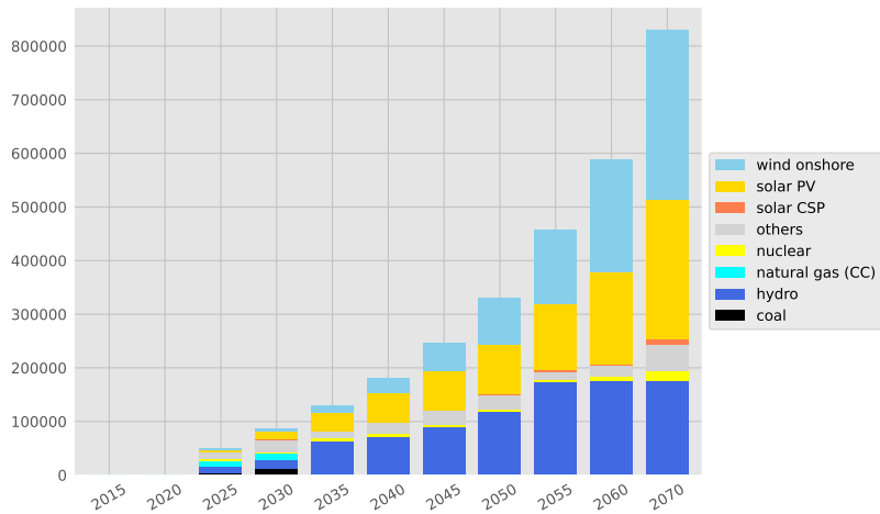
Power plant capacity (MW)
